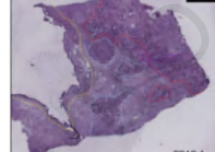
Cell-Type Score and Proportion Annotation Using Deconvolution-Based Algorithms
