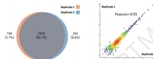
Site identification repeatability in two technical replicates
