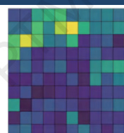
Visualization of Individual Differential Proteins
