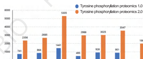
Comparison of tyrosine phosphorylation proteomics depths 1.0 and 2.0
