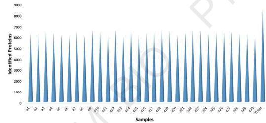
Deep Insight Blood+DIA Proteomics Reveals 8000+ Plasma Proteins
